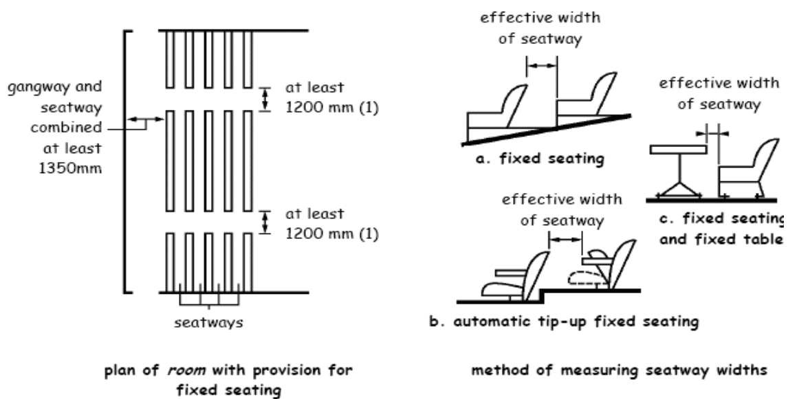
plan of room with provision for fixed seating
