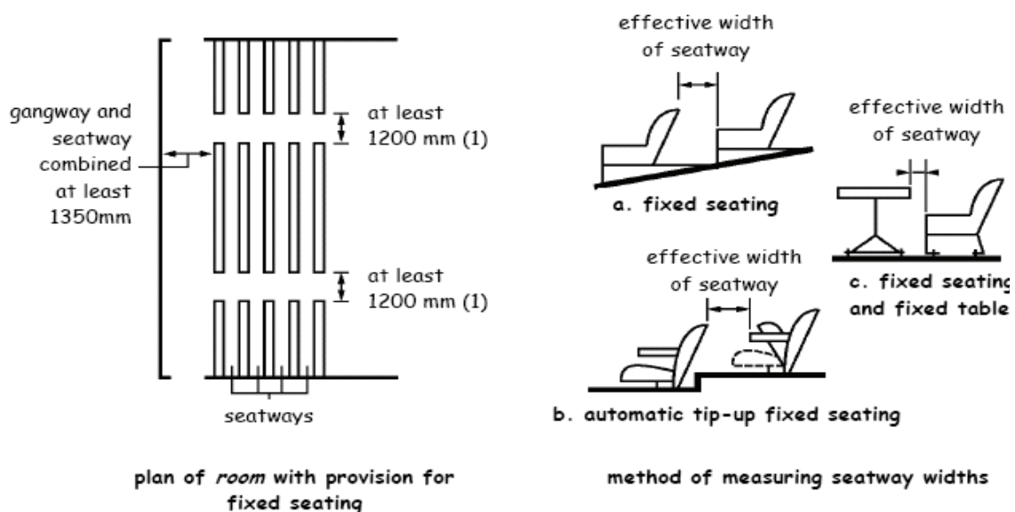
Minimum width of gangways & seatways in a room with fixed seating
